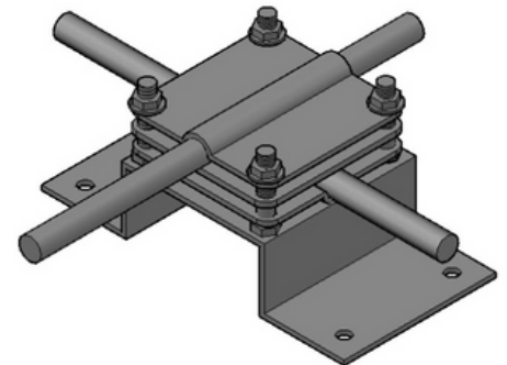
TOPRAKLAMA EK ELEMANI BAĞLANTI TABANI ELEMANI EARTHING CONNECTION BASE
