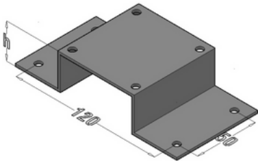
TOPRAKLAMA EK ELEMANI BAĞLANTI TABANI ELEMANI EARTHING CONNECTION BASE
