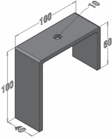
LAMBA AYAĞI - HARİCİ LAMBA AYAĞI LAMP SUPPORT - EXTERIOR LAMP SUPPORT
