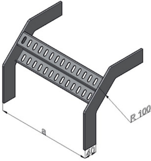
SİMETRİK DİŞ BÜKEY ELEMANLARI SYMMETRICAL TYPE OUTSIDE ELBOWS
