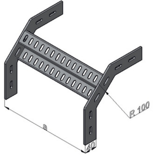
DELİKLİ TİP SİMETRİK DİŞ BÜKEY ELEMANLARI PERFORATED TYPE SYMMETRICAL OUTSIDE ELBOWS
